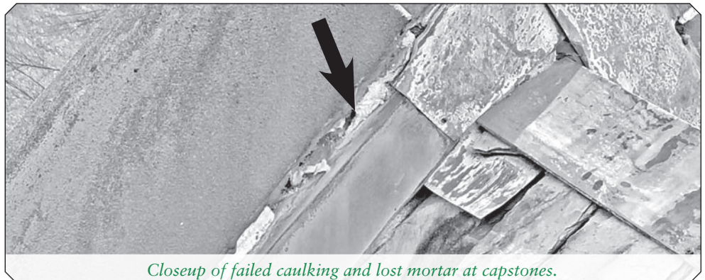
Gable flashing, mortar, and caulking failure at roof line masonry.
